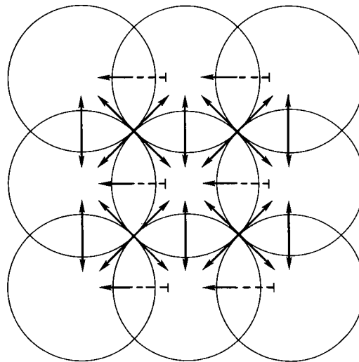
FIG. 18. Schematic representation of a neural mechanism for implementation of a pattern-motion detector relying on unoriented input. This mechanism requires lateral inhibitory neurons that are asymmetric and time delayed. It is formed by extension of a model of Barlow and Levick (7) type to 2 dimensions. Circles represent receptive fields of subunit neurons and aggregation of these fields represents receptive field of postsynaptic directionally selective neuron. There are time-delayed inhibitory interneurons (bold arrows) from each subunit neuron to all but 1 of adjacent subunits (dashed lines). Like simpler one-dimensional case, this model is normally most sensitive to motion in single direction where there are no lateral inhibitory interneurons, i.e., to right in this arrangement.
