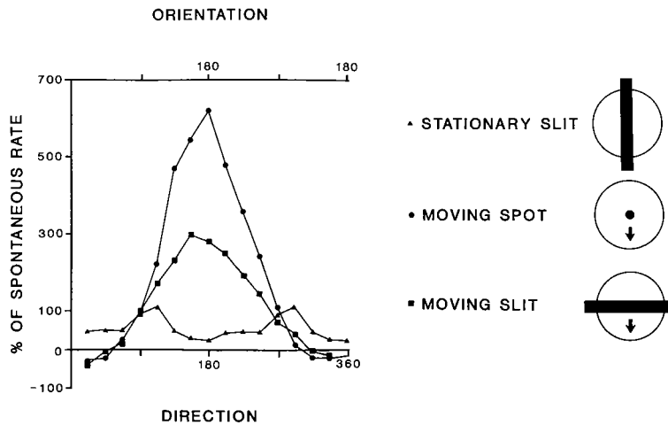
FIG. 6. Relationship between direction and orientation tuning that is characteristic of some type II MT neurons. Direction tuning for moving spot is similar to that for moving slit. Optimal orientation for stationary slit is shifted ~90° away from optimal direction of motion. This relationship, reflecting an orientation preference that is parallel to direction preference, is illustrated schematically at right. See also legend to Fig. 5.
