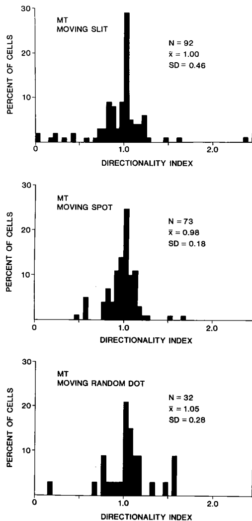
FIG. 13. Distributions of directionality index measure for moving slit (top), moving spot (center), and moving random-dot field (bottom) for neurons in area MT.
