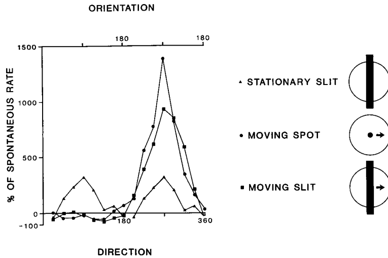
FIG. 5. Relationship between direction and orientation tuning that is characteristic of type I MT neurons. Responses (percent of spontaneous rate) are plotted on graph at left as a function of direction (lower axis) for moving stimuli and as a function of orientation (upper axis) for stationary stimuli. Direction tuning for moving spot is indicated by circles and that for moving slit is indicated by squares. Orientation tuning for stationary slit is indicated by triangles and 2 cycles are plotted to facilitate comparison with direction tuning. Alignment of peaks for moving and stationary stimuli reflects an orientation preference that is perpendicular to preferred direction for both types of moving stimuli. This relationship is illustrated schematically at right.
