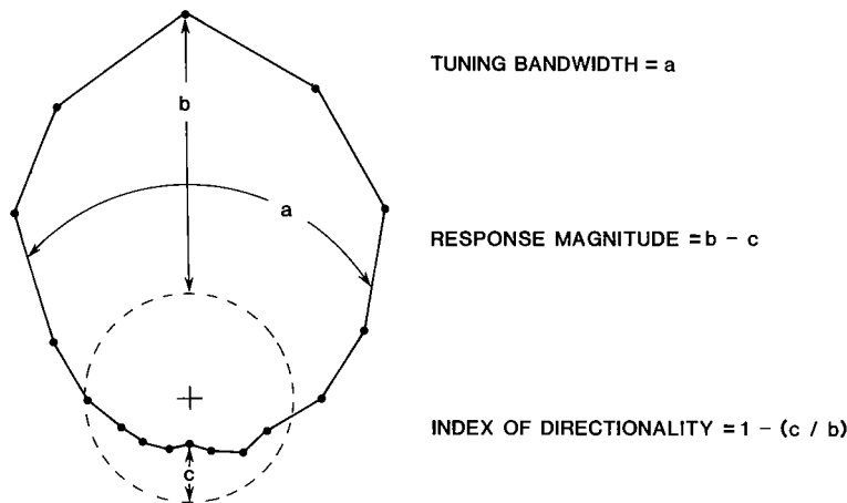
FIG. 8. Derivation of quantitative tuning measures. At left is a polar plot of a direction tuning curve. Broken line represents spontaneous activity level. Tuning bandwidth, a , is defined as full width of curve at a height one-half of distance between maximum and minimum responses. Differential response magnitude is difference between maximum ( b ) and minimum ( c ) response. Index of directionality is equal to 1 - (c/b) . See also legend to Fig. 1.
