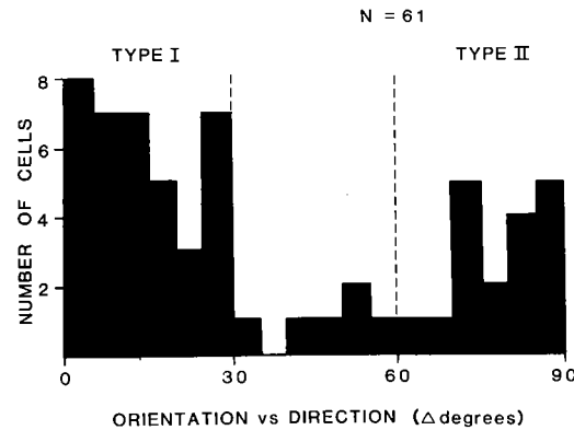
FIG. 4. Distribution of angular difference between optimal direction of motion and optimal orientation. Differences of 0^\circ reflect an orientation preference that is perpendicular to preferred direction of motion. Differences of 90^\circ reflect an orientation preference that is parallel to preferred direction of motion. Type I MT neurons (61%) are defined as those that have an optimal orientation roughly perpendicular to preferred direction of motion, i.e., a difference measure of less than 30^\circ . Type II neurons (29%) are defined as having an optimal orientation roughly parallel to preferred direction of motion, i.e., a difference measure greater than 60^\circ . Proportion of cells in these 2 groups differs significantly from a uniform distribution. Cells with difference measures between 30 and 60^\circ (10%) were not classified as type I or II.
