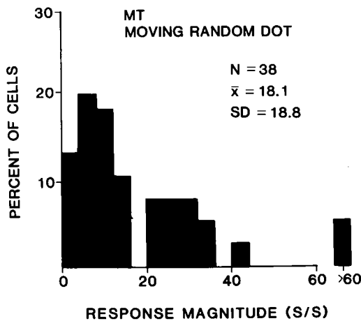
FIG. 11. Distributions of response magnitude measure for moving slit (top), moving spot (center), and moving random-dot field (bottom) for neurons in area MT.
