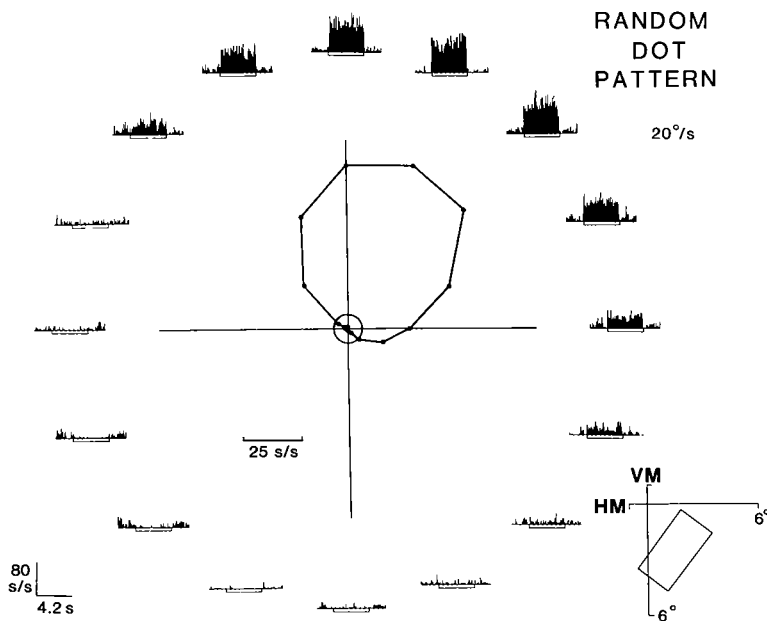
FIG. 1. Example of direction tuning of a typical MT neuron. Individual histograms represent responses summed over 5 trials to each of 16 directions of motion of a random-dot pattern moving at 20°/s. Line beneath each histogram indicates period of time during which stimulus was moving through receptive field (shown at lower right). In center, response for each direction is plotted on a polar graph. Radial axis represents response (measured as spikes per second), the polar axis represents direction of stimulus motion, and small circle represents level of spontaneous activity. Marked suppression of activity in direction 180° away from optimal is characteristic of many MT neurons. VM, vertical meridian, HM, horizontal meridian.
