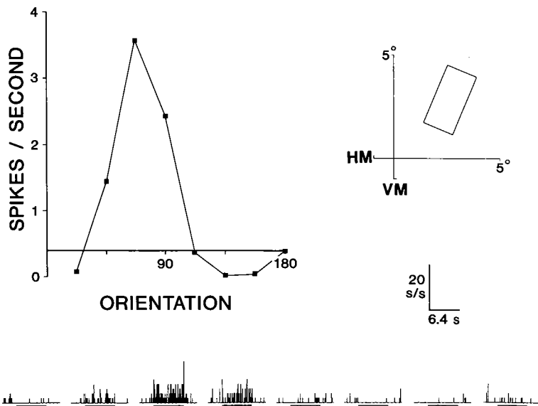
FIG. 3. Tuning of an MT neuron to orientation of a stationary flashed slit. This neuron exhibited a sustained response during stimulus exposure. See also legends to Figs. 1 and 2.
