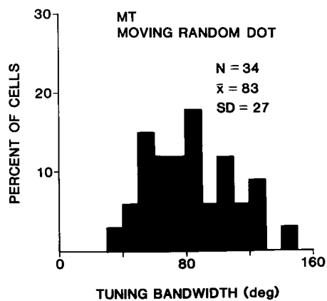
FIG. 10. Distributions of direction tuning bandwidth measure for moving slit (top), moving spot (center), and moving random-dot field (bottom) for neurons in area MT.
