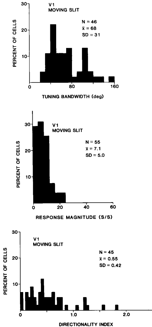
FIG. 15. Distributions of the moving-slit direction-tuning bandwidth (top), response magnitude (center) and directionality index (bottom) for neurons in area V1.
