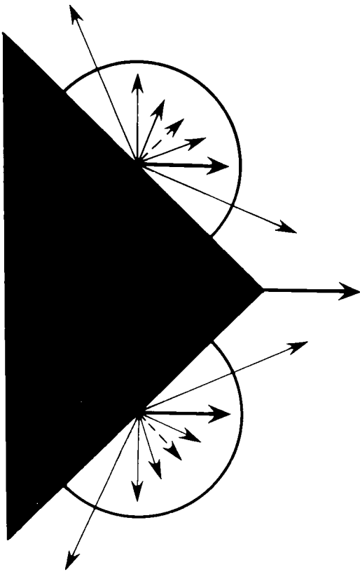
FIG. 17. "Velocity-space rule" solution to problem of extracting pattern motion (1). A simple two-dimensional pattern is formed from 2 oriented contours. Pattern has a direction and speed of motion indicated by velocity vector drawn at apex. When viewed through apertures (circles), each oriented contour appears to move along axis perpendicular to its orientation (dashed-line vector). Motion of each contour is consistent with a family of motions (a "velocity space" represented by set of velocity vectors associated with each contour) of pattern in which they are embedded. Direction and speed of motion of pattern can be determined by "intersection" of velocity-space vectors for each of 2 contours, i.e., single speed and direction of motion that is simultaneously consistent with motion of both oriented contours (indicated by bold vector for each contour).
