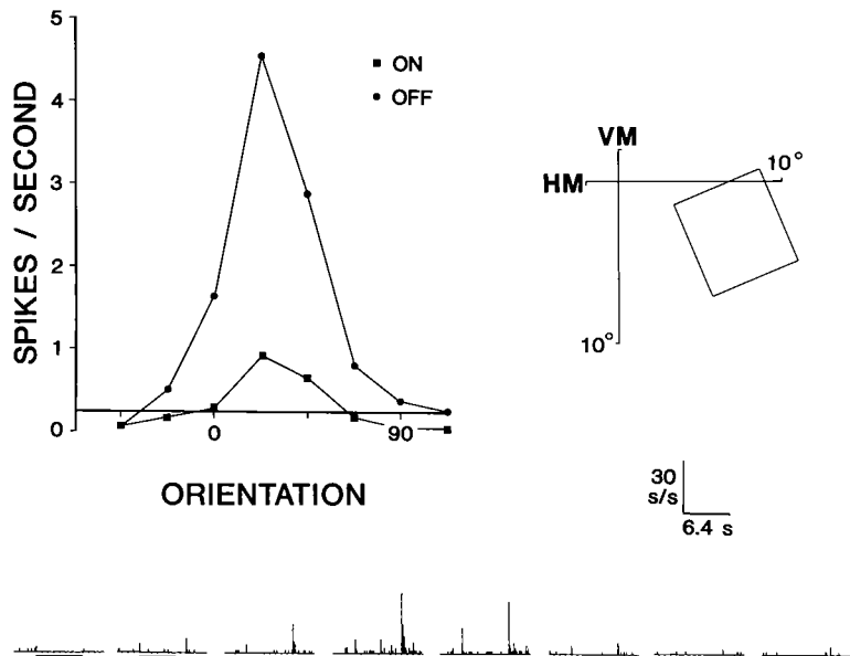
FIG. 2. Tuning of an MT neuron to orientation of a stationary flashed slit. This neuron exhibited a small transient "on" response and a larger "off" response. Histograms at bottom represent responses to 5 trials for each of 8 orientations. Both "on" and "off" responses are plotted as a function of orientation on graph at upper left. Horizontal line represents level of spontaneous activity. Receptive field is shown at upper right. See also legend to Fig. 1.
