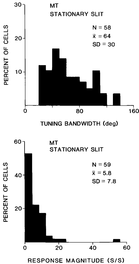
FIG. 14. Distributions of orientation-tuning bandwidth (top) and response magnitude (bottom) for stationary flashed slit ("on" response only) for neurons in area MT.
