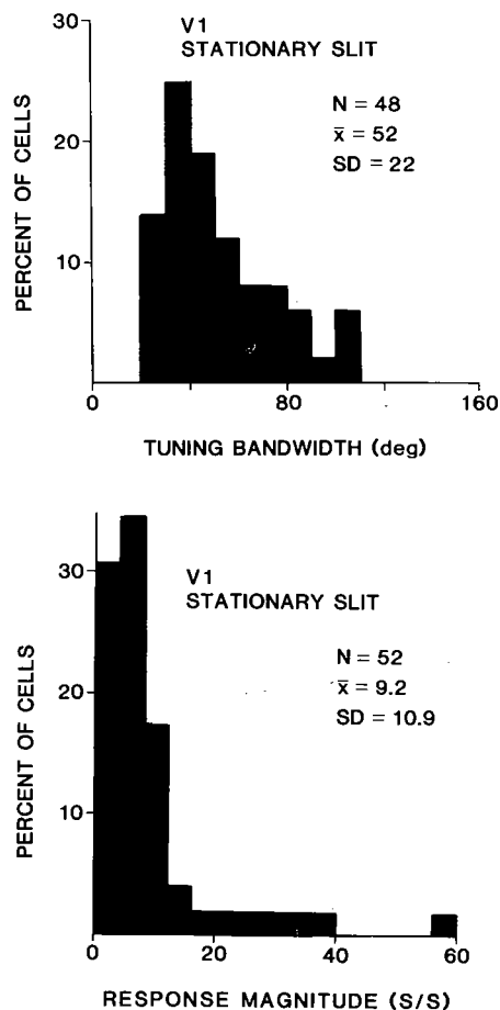
FIG. 16. Distributions of orientation-tuning bandwidth (top) and response magnitude (bottom) for stationary-flashed slit ("on" response only) for neurons in area V1.
