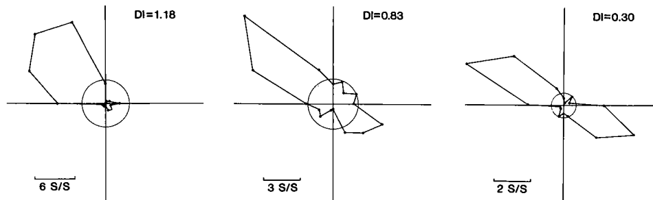
FIG. 12. Range of variation of direction selectivity along preferred axis of motion is illustrated by tuning curves obtained from 3 different MT neurons. Index of directionality, a measure of direction selectivity, is indicated for each curve. Average index of directionality for MT neurons (1.00) falls between strongly unidirectional curve at left and directionally biased curve at center. Stimulus for each curve shown here was a moving slit. See also legend to Fig. 1.
