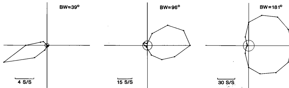
FIG. 9. Range of variation of direction-tuning bandwidth is illustrated by tuning curves obtained from 3 different MT neurons. Full-width half-maximum measures of tuning bandwidth are indicated for each curve. Direction-tuning bandwidth of center curve is representative of average for MT neurons. Stimulus for each curve shown here was a moving slit. See also legend to Fig. 1.
