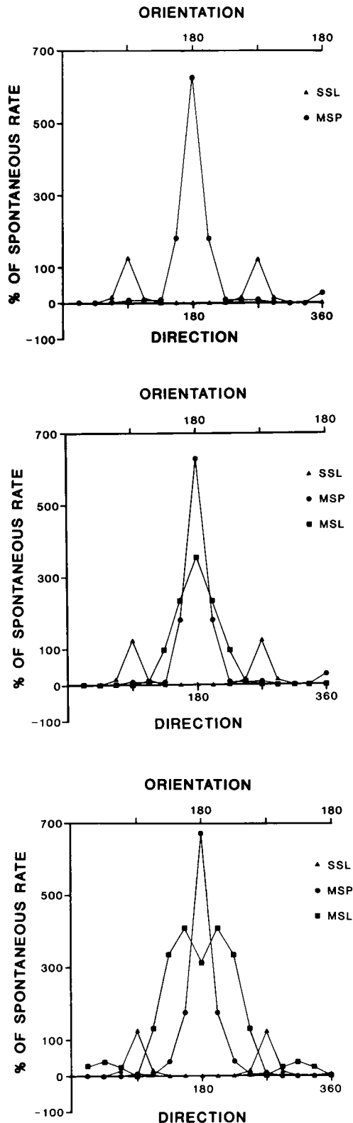
FIG. 19. Direction and orientation tuning from a computer simulation of a pattern-motion sensitive neuron. This simulation is based on a model that requires asymmetric lateral interconnections between nonorientation-selective inputs (see text and Fig. 18). Simulated output is plotted for 8 different orientations and 16 different directions. Both response scaling and "spontaneous activity" level (horizontal line) are arbitrarily chosen. Similarities to type II MT neurons are striking (cf. Figs. 6 and 7). Top: stationary slit (SSL) orientation tuning, indicated by triangles, is plotted twice to facilitate comparison with moving spot (MSP) direction tuning, indicated by circles. Like type II MT neurons, optimal orientation for a stationary slit deviates 90^\circ from optimal direction of motion, indicating an orientation preference parallel to direction preference. Center: like most type II MT neurons, direction tuning for a moving slit (MSL), indicated by squares, is similar to that for a moving spot and parallel to stationary-slit orientation preference. Bottom: like some type II MT neurons, moving-slit direction-tuning curve is bimodal, indicating 2 preferred directions that are symmetrical about that for moving spot and intermediate between moving spot direction preference and orientation preference. This simulation differs from that shown at center only by a one-third reduction in speed for moving stimuli.
