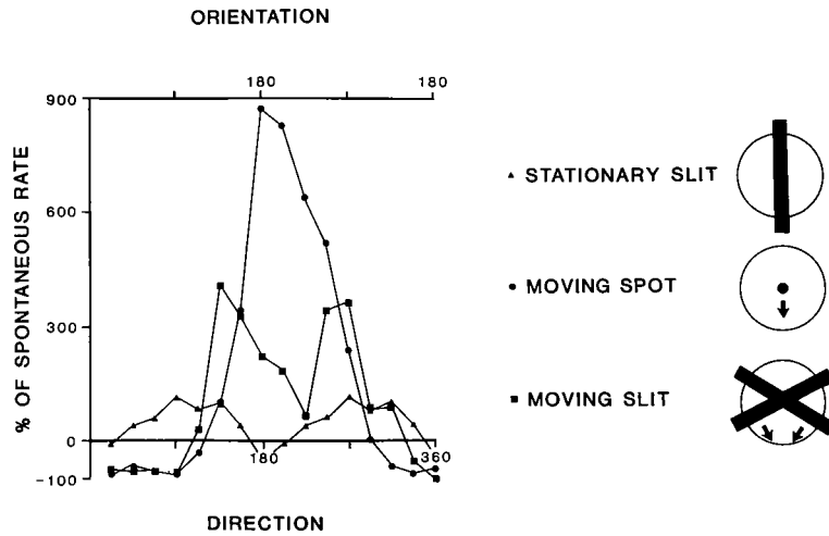
FIG. 7. Relationship between direction and orientation tuning that is characteristic of some type II MT neurons. Orientation preference for stationary slit is shifted \sim 90^\circ away from optimal direction for moving spot, reflecting an orientation preference parallel to preferred direction. Direction tuning curve for moving slit indicates 2 preferences that are symmetrical about single moving-spot preference and intermediate between moving-spot and stationary-slit preferences. These unusual relationships are illustrated schematically at right. See also legend to Fig. 5.
